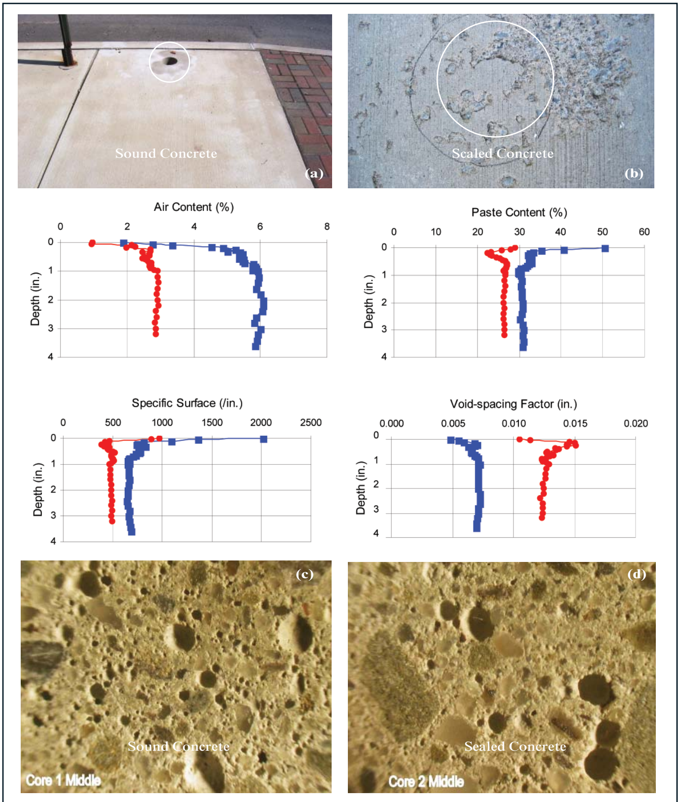
Fig. 2: Case study II: Scaling due to improper air entrainment (coarse air-void system with low air content and wide void spacing). Photos (a) and (b) show the surface conditions of panels where cores were taken; the graphs show profiles of air-void parameters in scaled (in red) and sound (in blue) concretes; and photos (c) and (d) show air-void systems in cross sections of sound and scaled cores. Note: 1 in. = 25.4 mm
